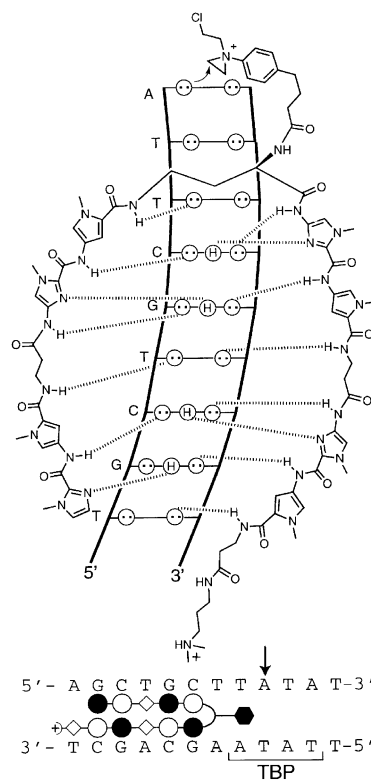
Figure 29. (top) Hydrogen-bonding model and alkylation mechanism of polyamide-CHL conjugate ImPy- \beta -ImPy-(R) CHL - \gamma -ImPy- \beta -ImPy- \beta -Dp (2) bound to the minor groove of 5'-AGCTGCT-3'. Circles with two dots represent the lone pairs of N3 purines and O2 of pyrimidines. Circles containing an H represent the N2 hydrogens of guanines. Model of polyamide conjugate bound to the match site 5'-AGCTGCT-3'. Black and white circles represent imidazole (Im) and pyrrole (Py) polyamide rings, respectively. Diamonds and hexagon represent \beta alanine ( \beta ) and CHL, respectively. (R)-2,4-diaminobutyric acid [(R) \gamma ] and dimethylamino-propylamide (Dp) are depicted as a curved line and a plus sign, respectively. TBP, TATA box binding region.
