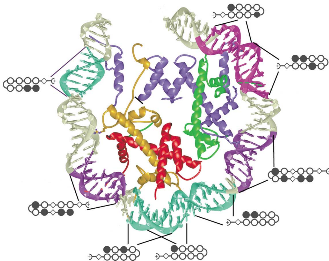
Figure 33. Polyamide binding to nucleosomal DNA. Ribbon diagram of one half of the nucleosome core particle (73 bp of DNA and associated proteins). H3 is shown in blue, H4 in green, H2A in yellow, H2B in red. Polyamide binding sites are shown as indicated.
