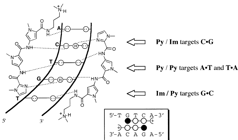
Figure 11. Model for antiparallel dimer ImPyPy binding 5'-TGTCA-3'. Unsymmetrical pair Im/Py distinguishes GC from CG and both from AT and TA.
