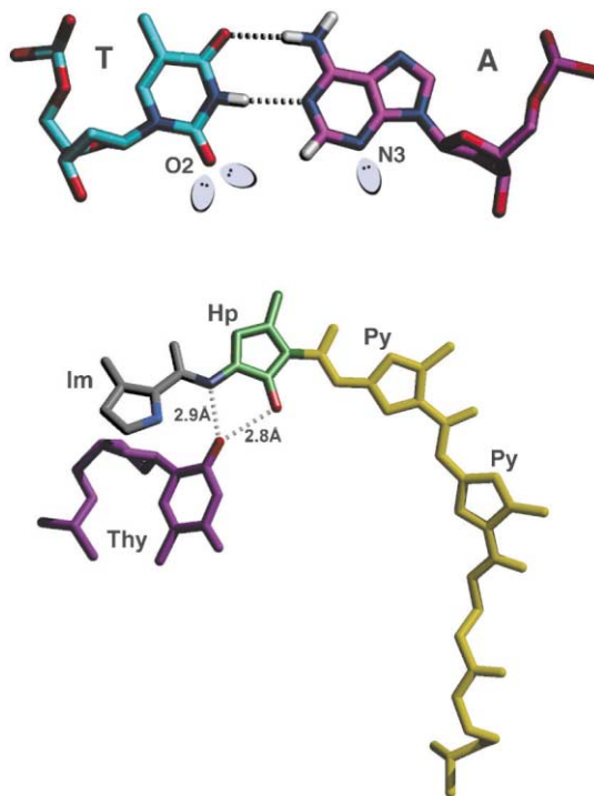
Figure 27. (top) Anatomy of the T•A base pair. Lone pair electron in the minor groove are shown as ovals and the Watson–Crick hydrogen bonds of the base pair as dotted lines. (bottom) The hydrogen bonds between ImHpPyPy and one strand of DNA, indicated by dashed lines. Note the two hydrogen bonds between Hp and O2 of T.
