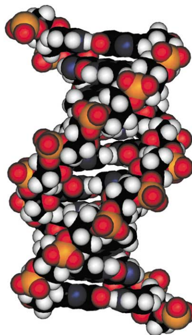
Figure 1. The DNA Helix.
