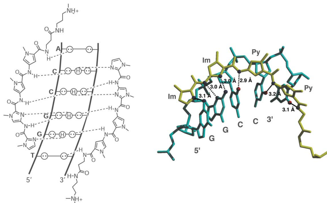
Figure 19. (left) Model of the polyamide bound as an antiparallel head to tail dimer. (right) Isolated view of one of the ImImPyPy-β-Dp molecules and hydrogen bonds with the adjacent DNA strand. The hydrogen bond lengths given are the average of the ncs-related strands.
