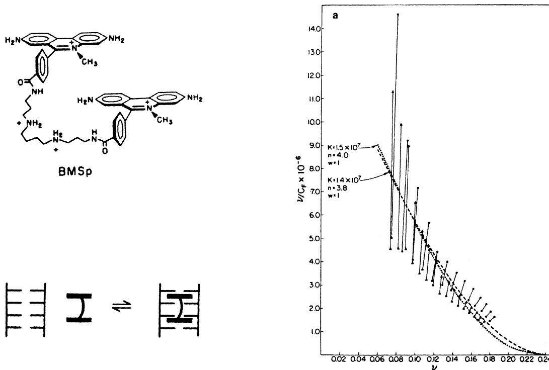
Figure 3. Bis(methidium) spermine, a synthetic bisintercalator, binds with high affinity to DNA.
