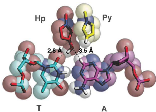
Figure 26. Space-filling model of the Hp/Py pair interaction with the T•A base pair shows that the Hp-OH tightly fits the cleft formed by the adenine C2H.
