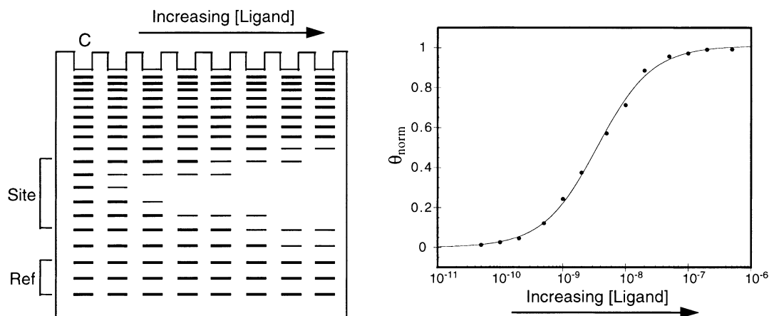
Figure 14. Quantitative footprinting titration analyses. (left) Cleavage pattern generated by quantitative DNaseI footprinting titration on a 3' end-labeled DNA fragment in the presence of increasing ligand concentration (right) Langmuir binding titration isotherm obtained from DNaseI data.
