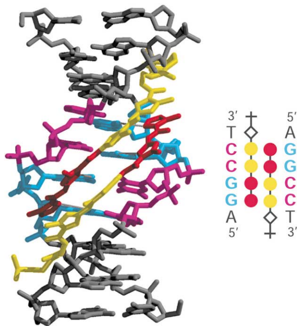
Figure 18. Stereodiagram of the polyamide-DNA complex (ImImPyPy-β-Dp) 2 •5'CCAGGCCTGG-3'. (Im-N-methylimidazole carboxamide, Py=N-methylpyrrole carboxamide, β=β-alanine, Dp=dimethylaminopripylamide).
