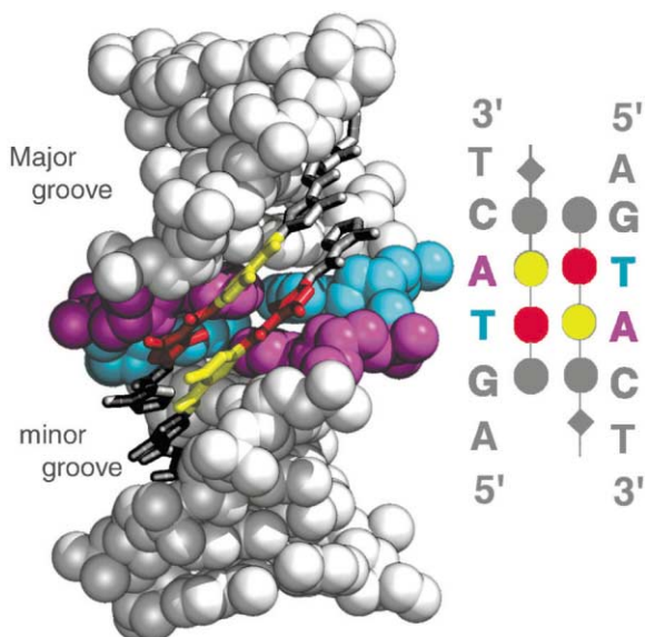
Figure 25. Space-filling model of (\text{ImHpPyPy})_2 \cdot 5'\text{-CCAGTACTGG-}3' . Adenosine is purple and thymidine cyan. The Hp is red and the Py paired with it is yellow.
