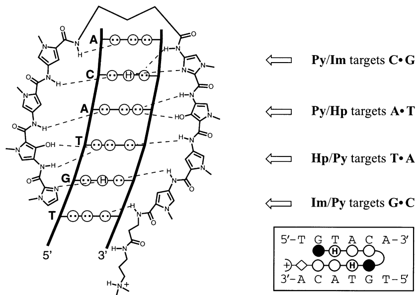
Figure 28. Molecular recognition of the minor groove of DNA. Minor groove hydrogen bonding patterns of Watson–Crick bps. Circles with dots represent long pairs of N(3) and O(2) of pyrimidines, and circles containing an H represent the 2-amino group of guanine. The R group represents the sugar-phosphate backbone of DNA. Binding model for the complex formed between ImHpPyPy- \gamma -ImHpPyPy- \beta -Dp and a 5'-TGTACA-3' sequence. Hydrogen bonds are shown as dashed lines. Im is black circles, Py is open circle and Hp is open circle with H.
