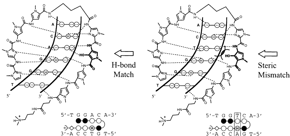
Figure 24. Models for Py/Hp binding AT, but not TA. (left) the Hp ring forms two hydrogen bonds with O2 of T and the hydroxyl fits in the cleft between A and T. (right) The Hp-OH has a steric clash with the A of the TA base pair.
