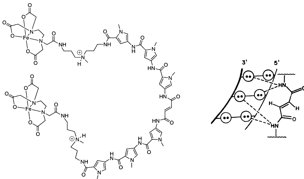
Figure 6. Distamycin dimer binds 9 base pairs of A,T rich DNA.
