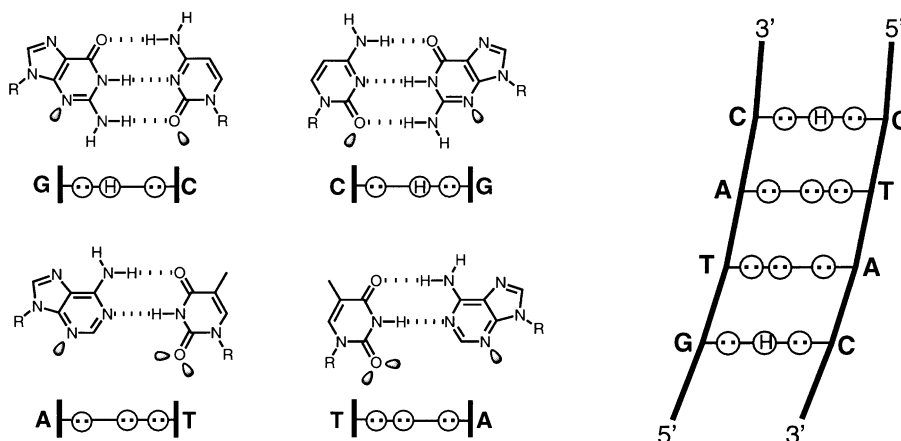
Figure 4. Molecular recognition of the minor groove of DNA. Minor groove hydrogen bonding patterns of Watson–Crick base pairs. Circles with dots represent lone pairs of N(3) of purines and O(2) of pyrimidines, and circles containing an H represent the 2-amino group of guanine.
