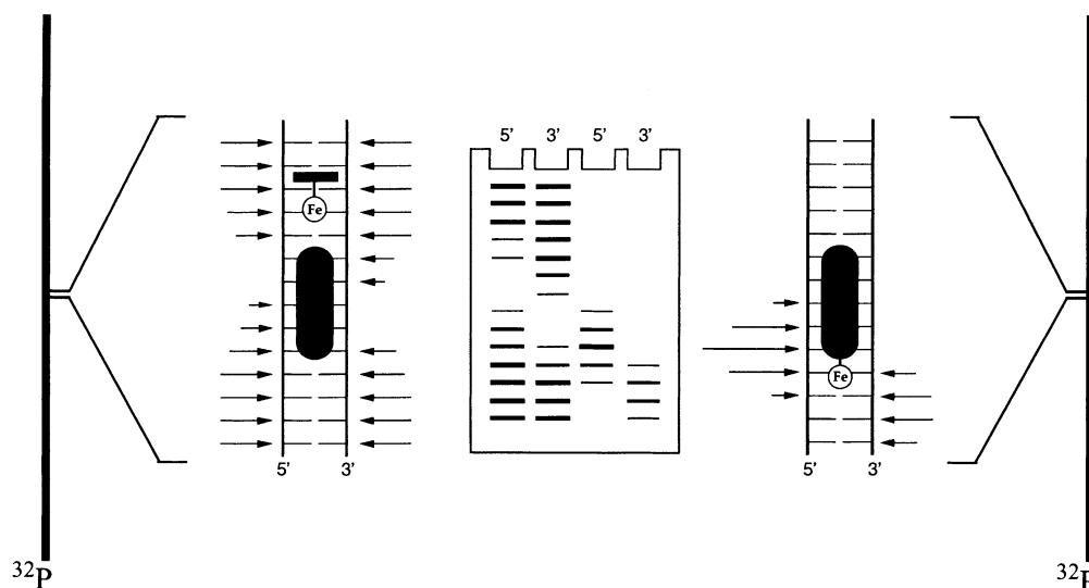
Figure 5. Schematic of (left) MPE•Fe(II) footprinting and (right) affinity cleavage techniques. (center) DNA cleavage products obtained on a denaturing gel with DNA end-labeled either the 5' or 3' strands are shown.
