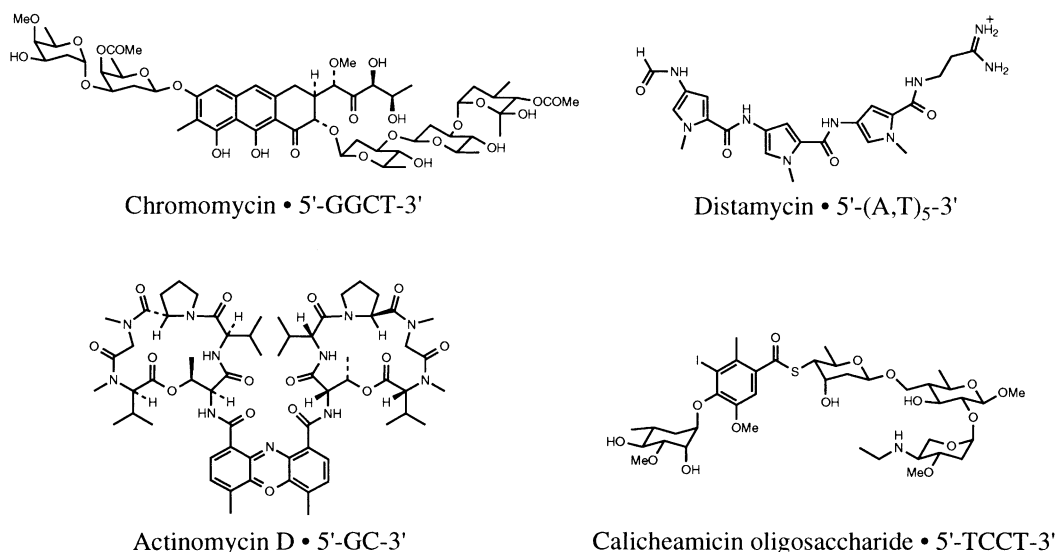
Figure 2. Natural products which bind DNA.
