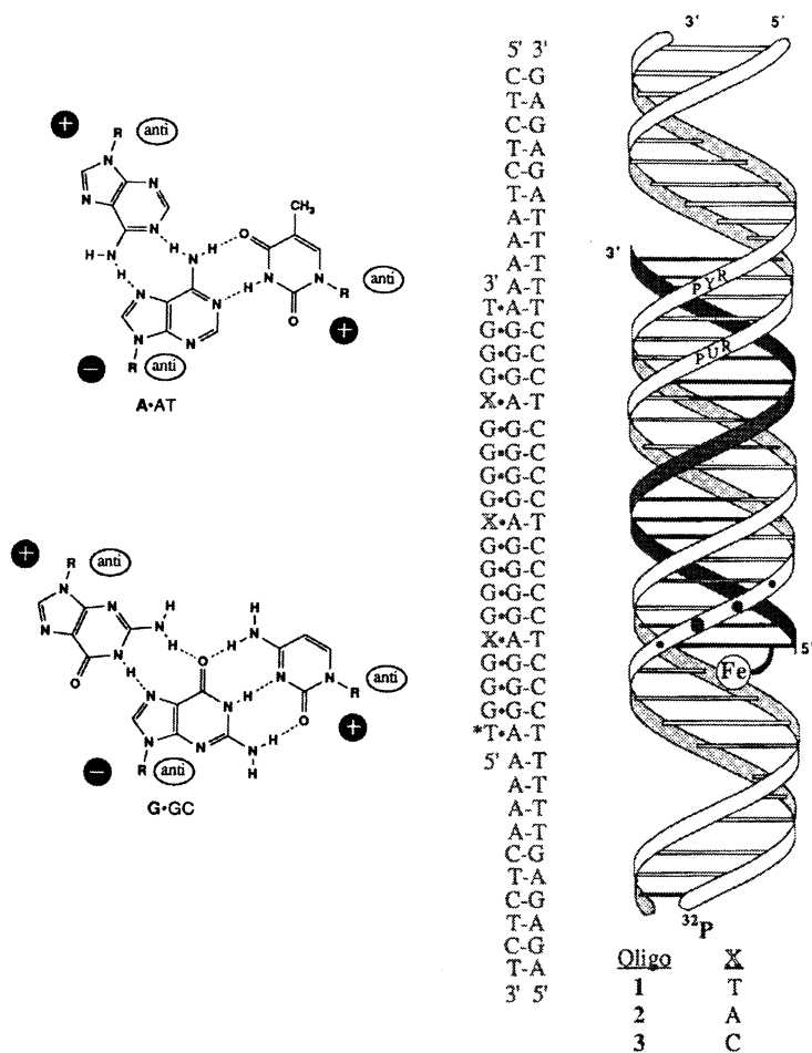
Figure 8. The purine triple helix motif. Isomorphous base triplets of AAT and GGC where the third strand is antiparallel to the purine Watson–Crick strand. Plus and minus indicate relative polarities of the phosphate–deoxyribose backbones.
