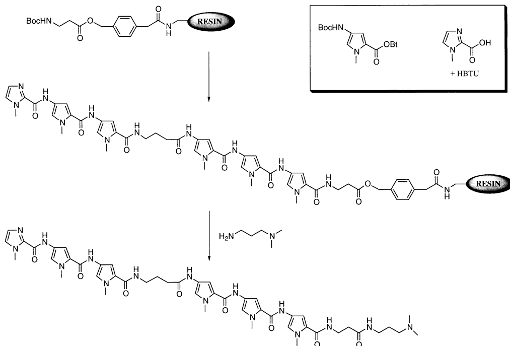
Figure 13. Solid phase synthesis of polyamides.
