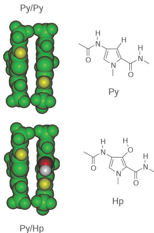
Figure 23. (top) Space filling model of the symmetrical Py/Py side-by-side antiparallel pair. (bottom) Space filling model of the unsymmetrical Py/Hp pair both viewed from the floor of the DNA helix.
