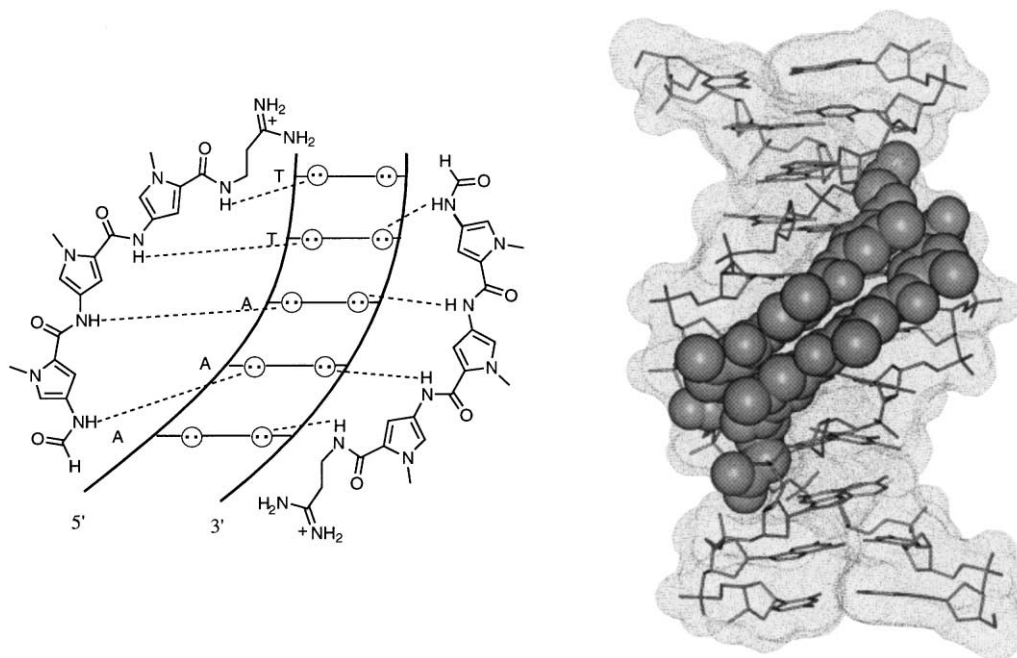
Figure 10. NMR structure of 2:1 complex of distamycin-DNA complex.
