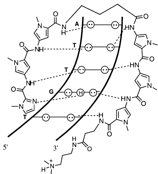
Figure 12. The hairpin motif. The amino and carboxy terminus of the antiparallel dimers are connected by \gamma -aminobutyric acid ( \gamma ).
