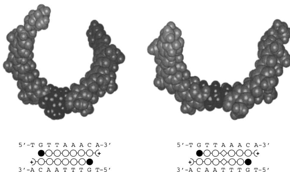
Figure 22. Space filling model of seven ring, ImPyPyPyPyPyPy-DP (left) and of 3-β-3 motif, ImPyPy-β-PyPyP-Dp (right). The 3-β-3 dimer curvature is lower than that of 3-Py-3 and fits better with the shape of the DNA helix.
