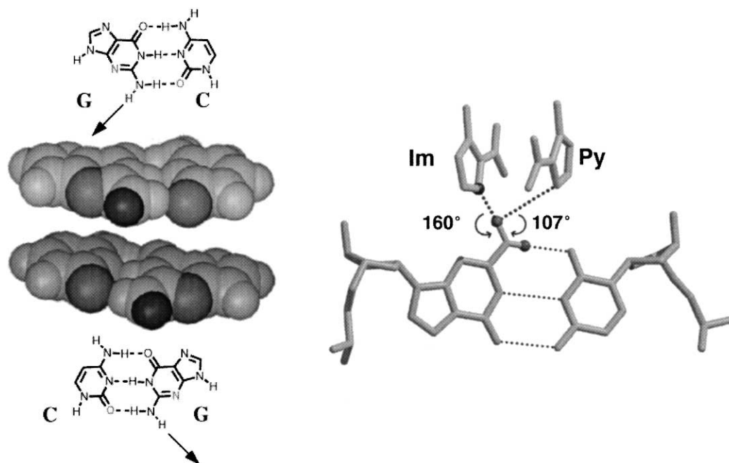
Figure 20. (left) Space filling model of GC versus CG. Note the exocyclic N-H of guanine points to one side of the minor groove. (right) Geometry of the Im-Py pair interacting with the G5•C16 base pair. An imidazole on the cytosine side of the base pair would be unable to form an optimum hydrogen bond with the hydrogen at the guanine exocyclic amine. This allows the Im-Py pair to discriminate the G•C base pair from C•G.
