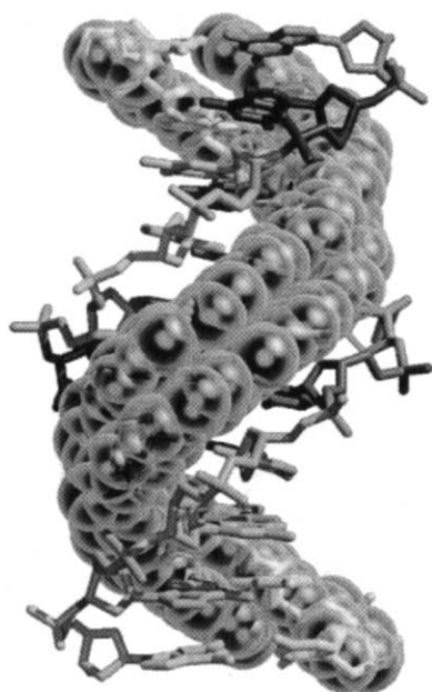
Figure 21. An extended polyamide helix. Least squares minimized, mean coordinates for a polyamide monomer were translated and rotated by the parameters of the polyamide helix. After a period of approximately seven residues, the 14 great twist of the polyamide with respect to B-form DNA manifests as clash with the walls of the minor groove.
